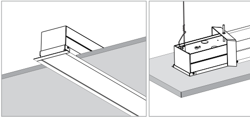
RT1: Mount by flanged trim and bracket in Dry ceiling
