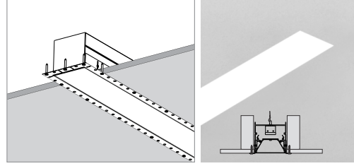
RS: Mount by trimless flanged kit and need plastering in Dry ceiling
