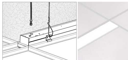
RH: Mount by T-grid hooks to secure in T-grid ceiling / Drop ceiling
