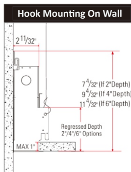
2.3" Width Version(Regressed Version)
