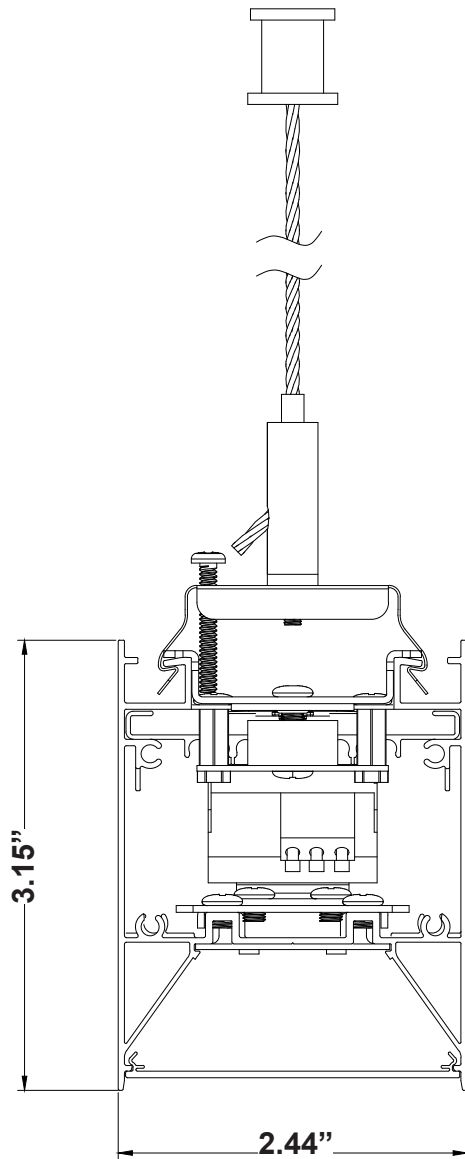
DIRECT LIGHT CROSS SECTION
