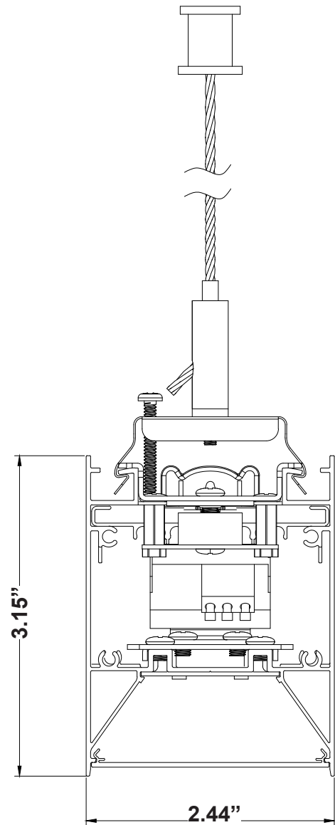
DIRECT/INDIRECT LIGHT CROSS SECTION
