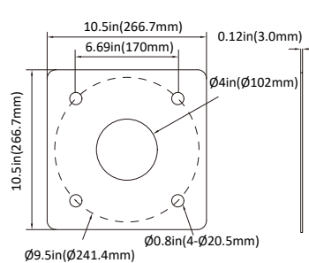
4" Screw Positioning Plate
