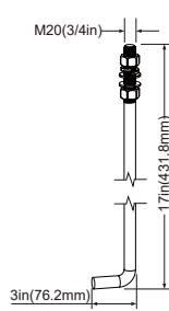
A1 Anchor Bolt Suit for 10ft, 15ft, 20ft
