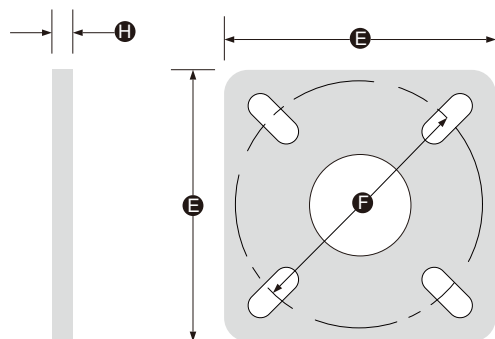
Base Plate with Slots or Holes
