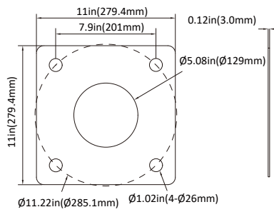
5" Screw Positioning Plate
