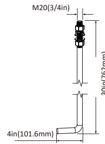
A2 Anchor Bolt Suit for 25ft
