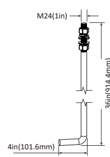
A3 Anchor Bolt Suit for 30ft
