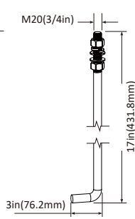
A1 Anchor Bolt Suit for 10ft, 15ft, 20ft
