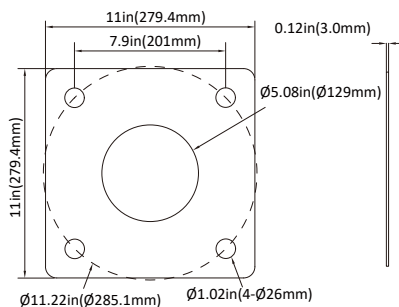
5" Screw Positioning Plate
