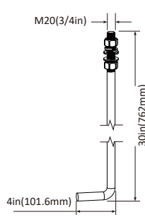
A2 Anchor Bolt Suit for 25ft
