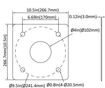
4" Screw Positioning Plate
