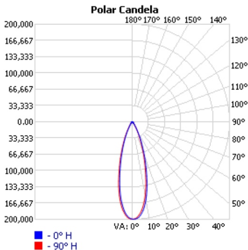
JHM-460W-40K-30D-P
