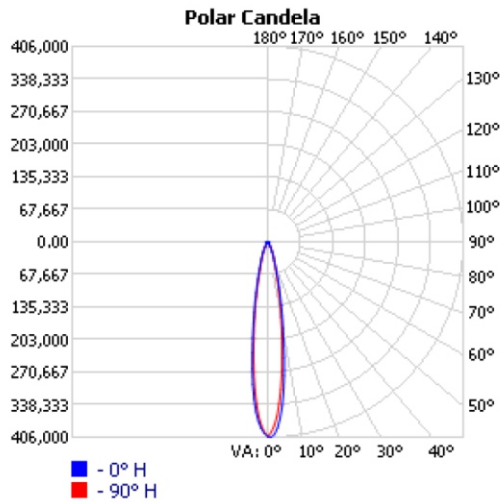
JHM-460W-40K-15D-P
