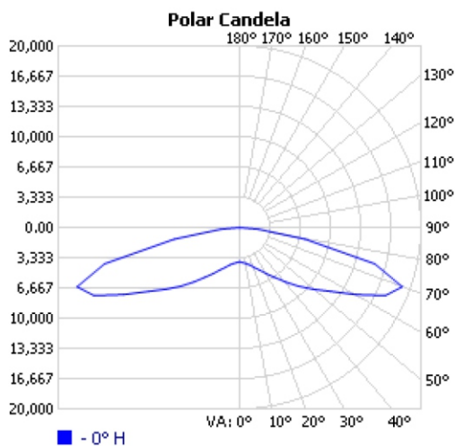
JHM-460W-40K-T5
