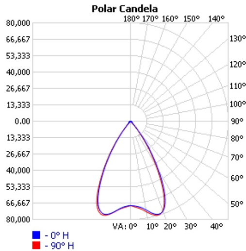
JHM-460W-40K-60D-P
