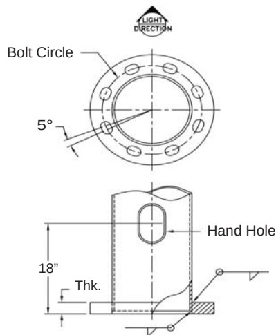
Base Plate Detail
