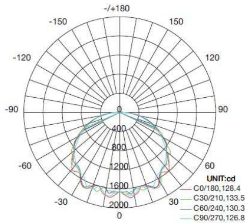
PVR-45W Luminous Intensity Distribution Diagram
