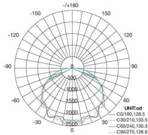
PVR-65W Luminous Intensity Distribution Diagram
