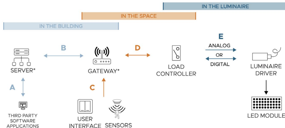
Centrally Networked Control System (Pacific Northwest National Laboratory)
